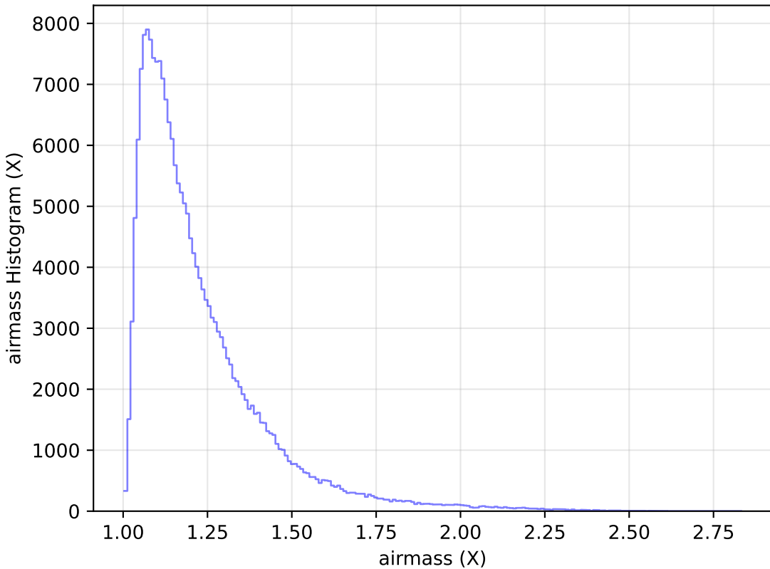
baseline_v2.1_10yrs All sky g band: airmass Histogram
