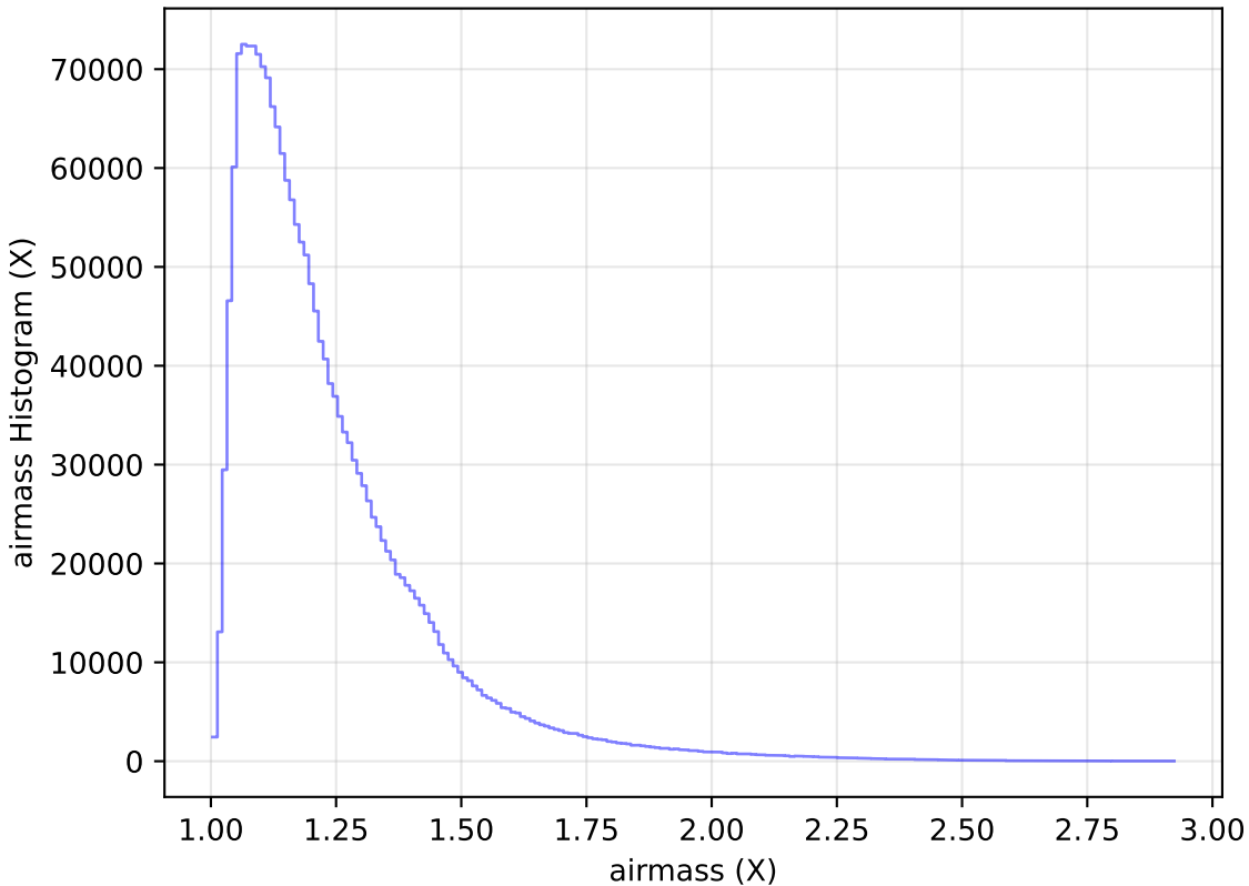
baseline_v2.1_10yrs All sky all bands: airmass Histogram
