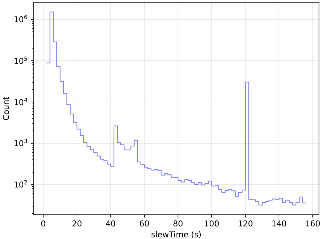
baseline_v2.1_10yrs All visits: Slew Time Histogram
