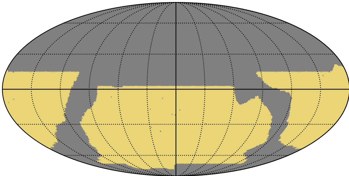
baseline_v2.1_10yrs WFD: RapidRevisits
