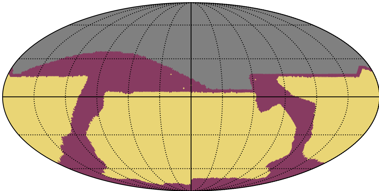
baseline_v2.1_10yrs All sky: RapidRevisits
