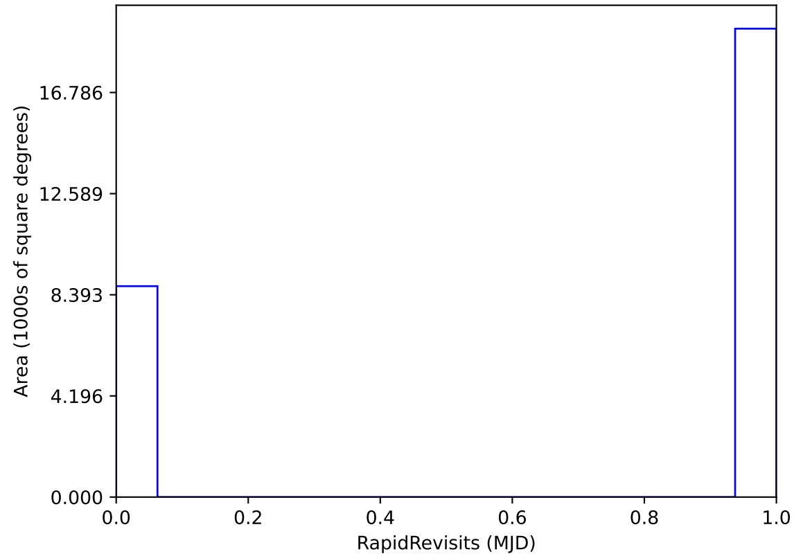
baseline_v2.1_10yrs All sky: RapidRevisits
