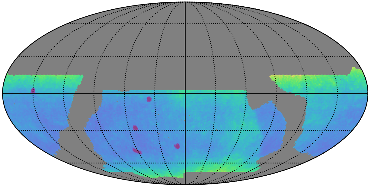
baseline_v2.1_10yrs WFD: Proper Motion Uncert @ 24.0
