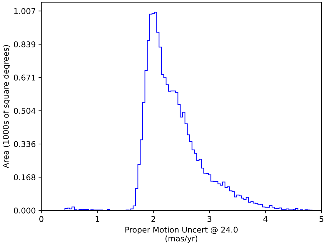
baseline_v2.1_10yrs WFD: Proper Motion Uncert @ 24.0
