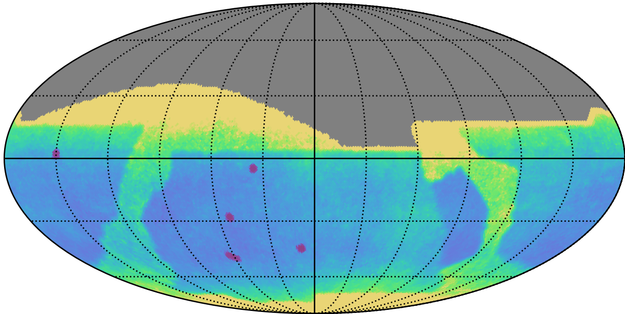
baseline_v2.1_10yrs All sky: Proper Motion Uncert @ 24.0
