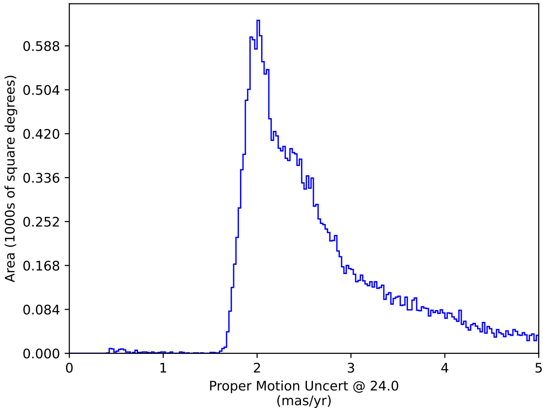
baseline_v2.1_10yrs All sky: Proper Motion Uncert @ 24.0
