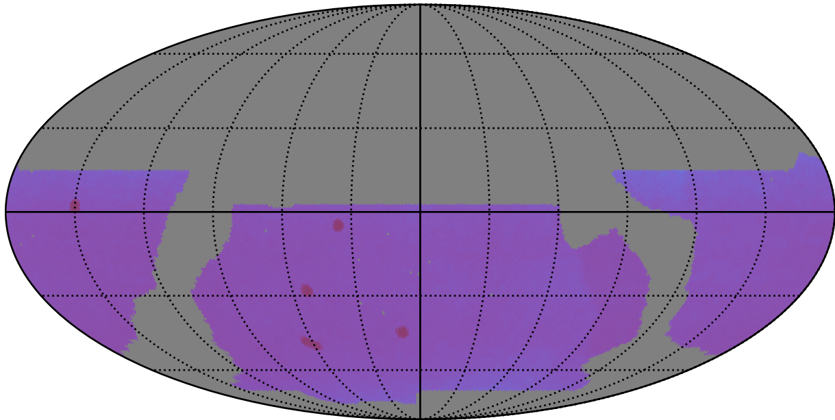
baseline_v2.1_10yrs WFD: Proper Motion Uncert @ 20.5
