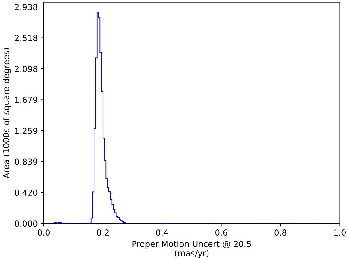
baseline_v2.1_10yrs WFD: Proper Motion Uncert @ 20.5
