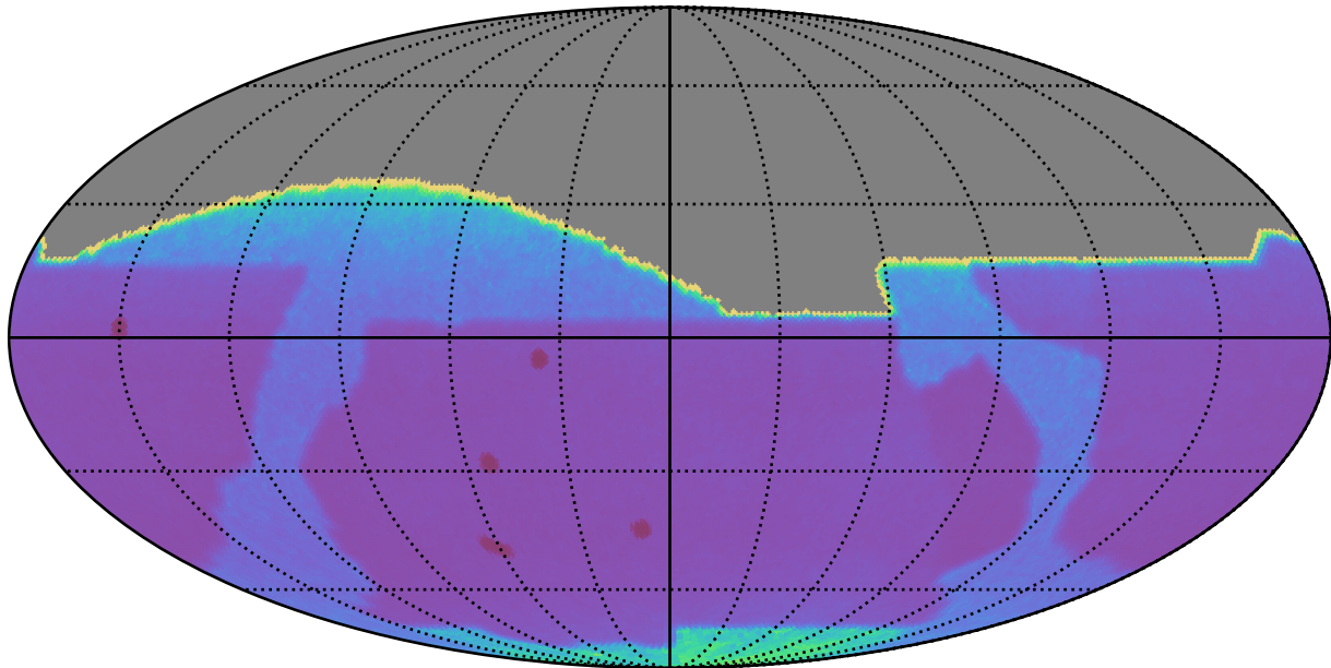
baseline_v2.1_10yrs All sky: Proper Motion Uncert @ 20.5
