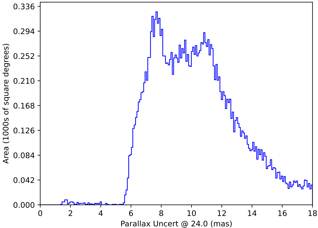
baseline_v2.1_10yrs All sky: Parallax Uncert @ 24.0
