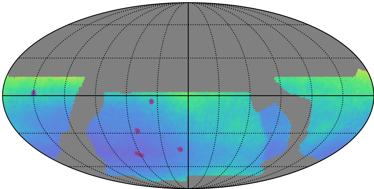
baseline_v2.1_10yrs WFD: Parallax Uncert @ 22.4
