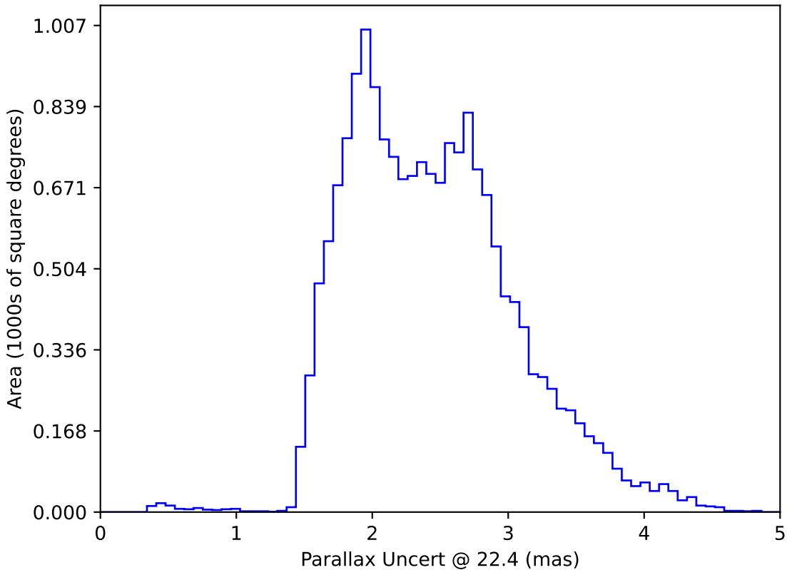
baseline_v2.1_10yrs WFD: Parallax Uncert @ 22.4
