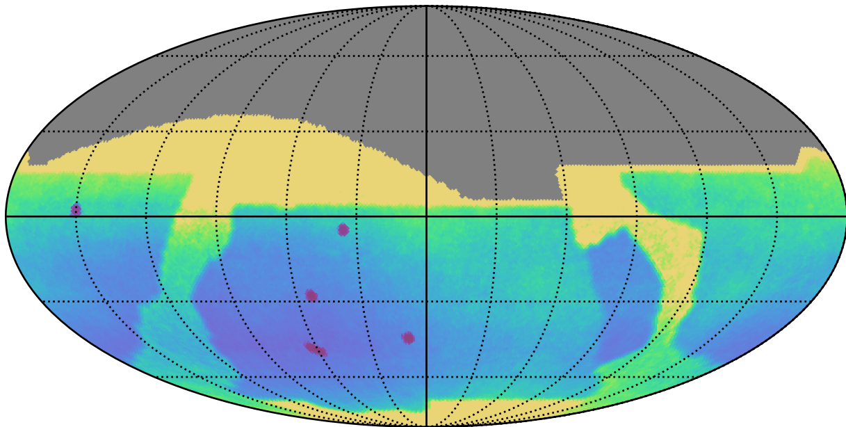
baseline_v2.1_10yrs All sky: Parallax Uncert @ 22.4
