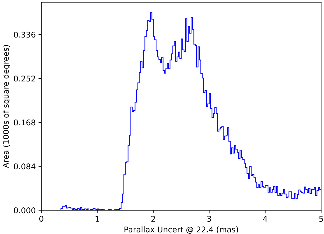
baseline_v2.1_10yrs All sky: Parallax Uncert @ 22.4
