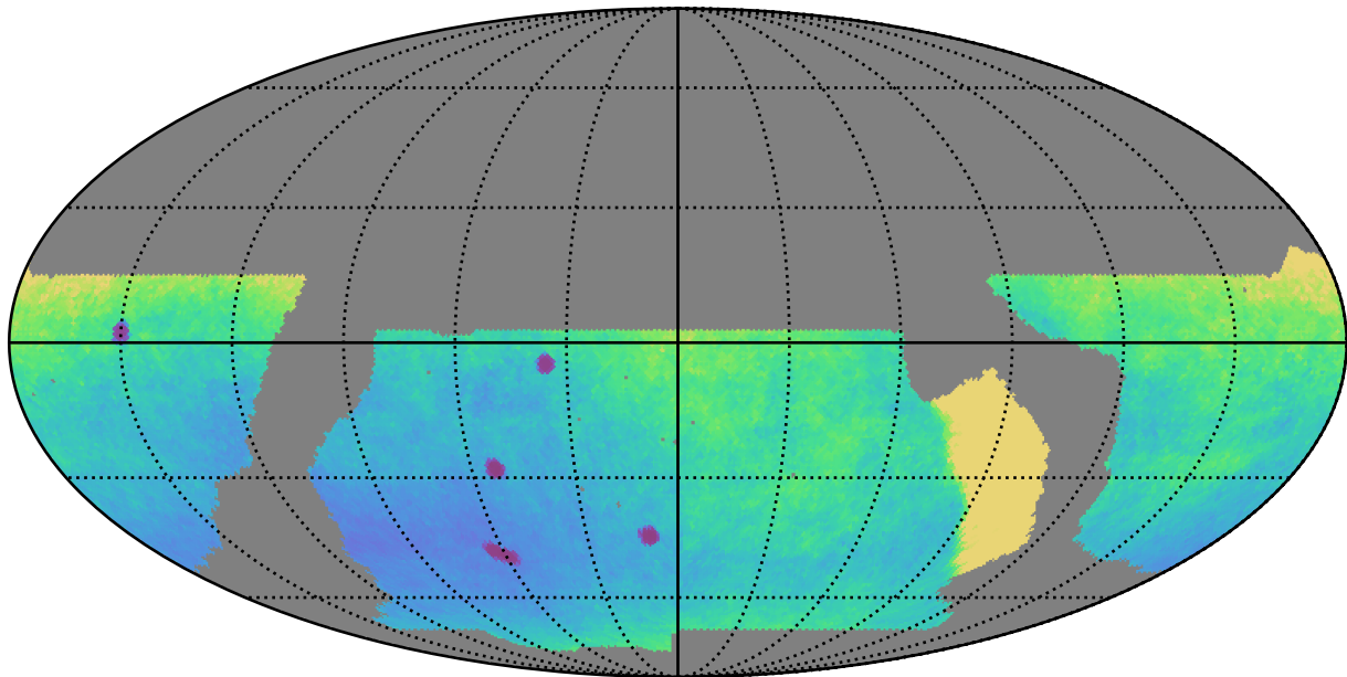
baseline_v2.1_10yrs WFD y band only: Parallax Uncert @ 21.3
