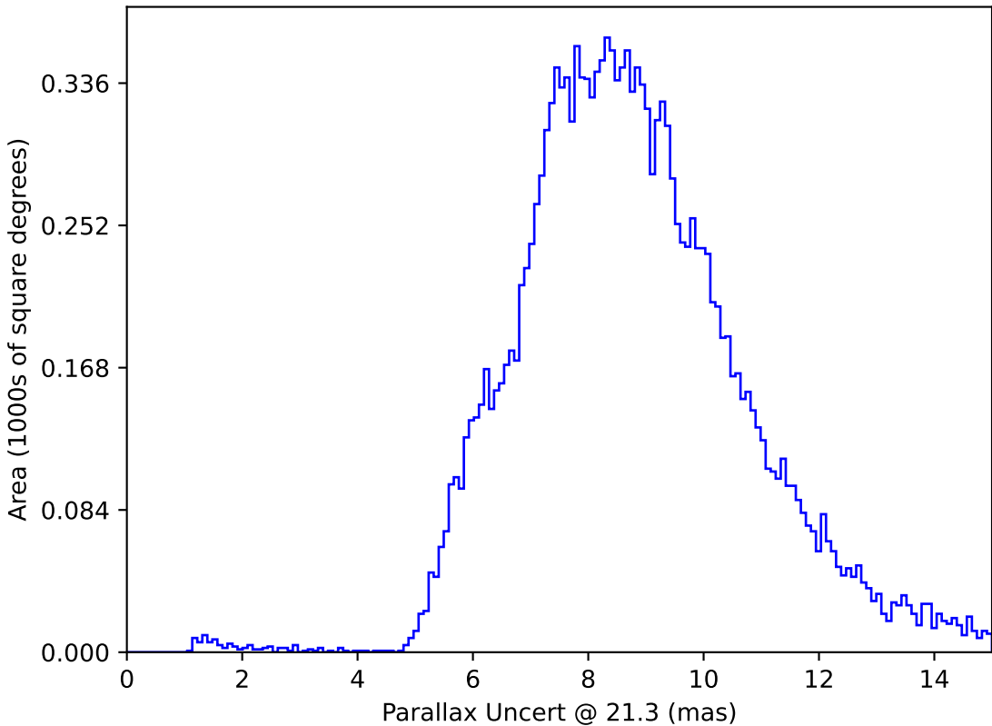
baseline_v2.1_10yrs WFD y band only: Parallax Uncert @ 21.3
