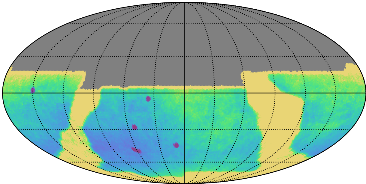
baseline_v2.1_10yrs All sky y band only: Parallax Uncert @ 21.3
