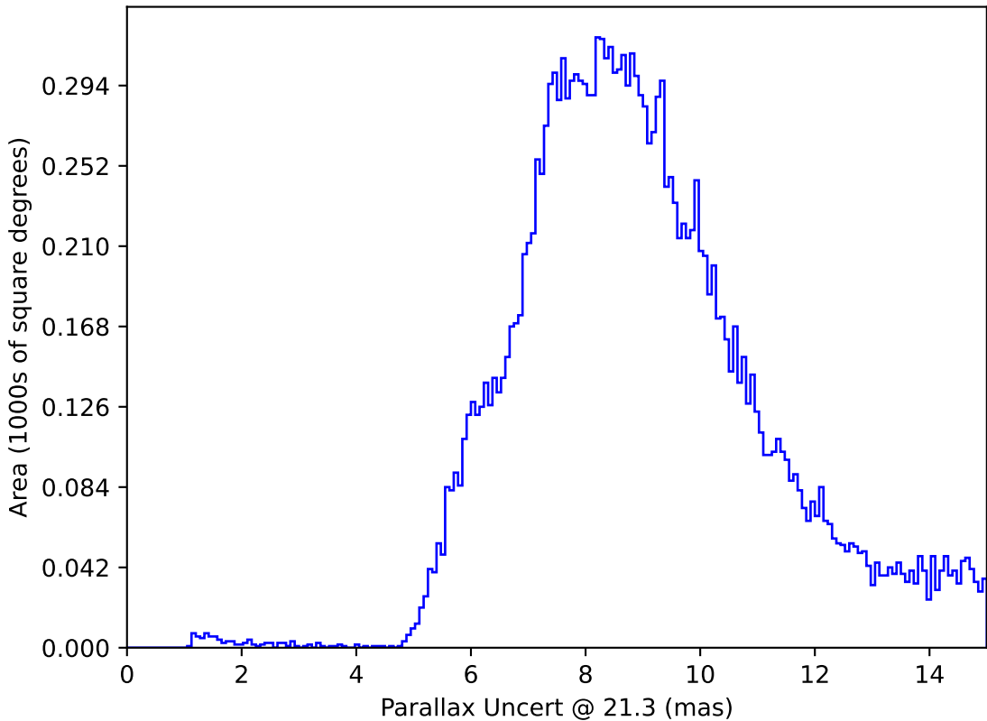
baseline_v2.1_10yrs All sky y band only: Parallax Uncert @ 21.3
