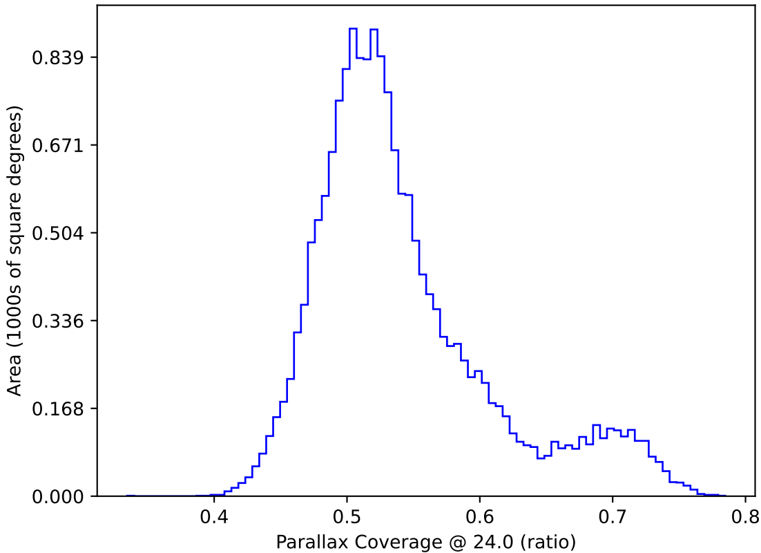
baseline_v2.1_10yrs WFD: Parallax Coverage @ 24.0
