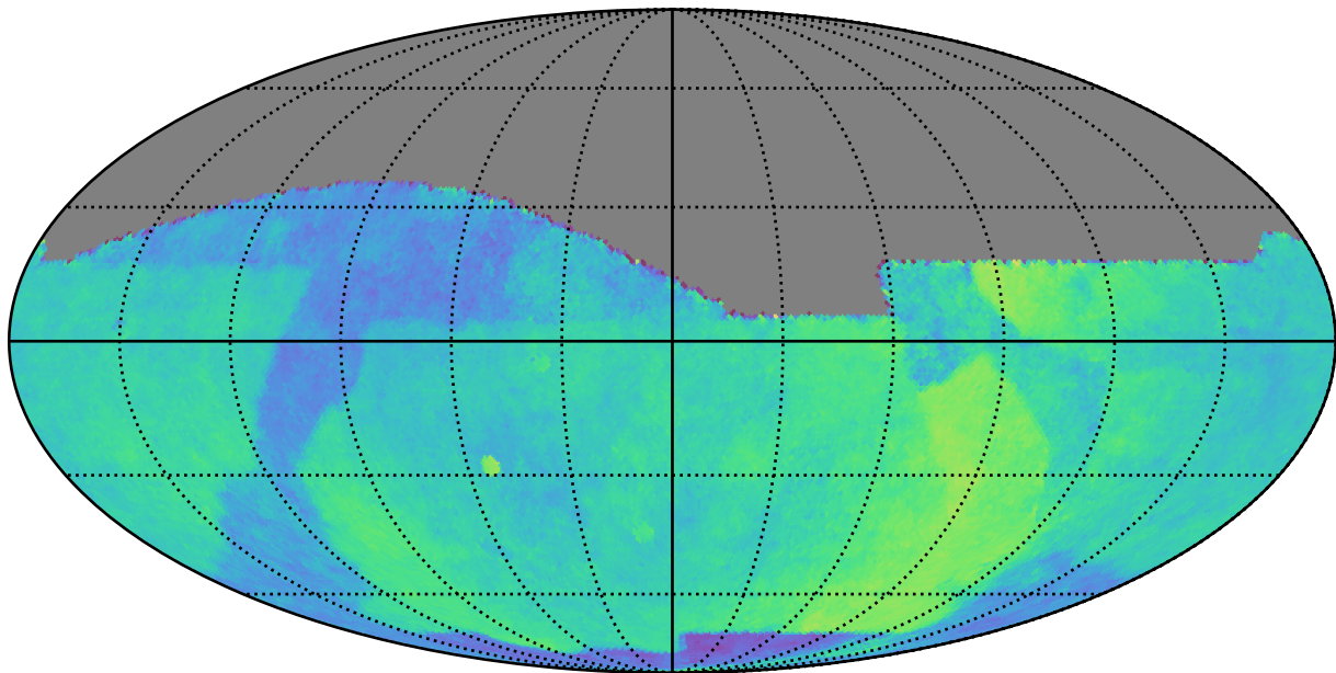
baseline_v2.1_10yrs All sky: Parallax Coverage @ 24.0
