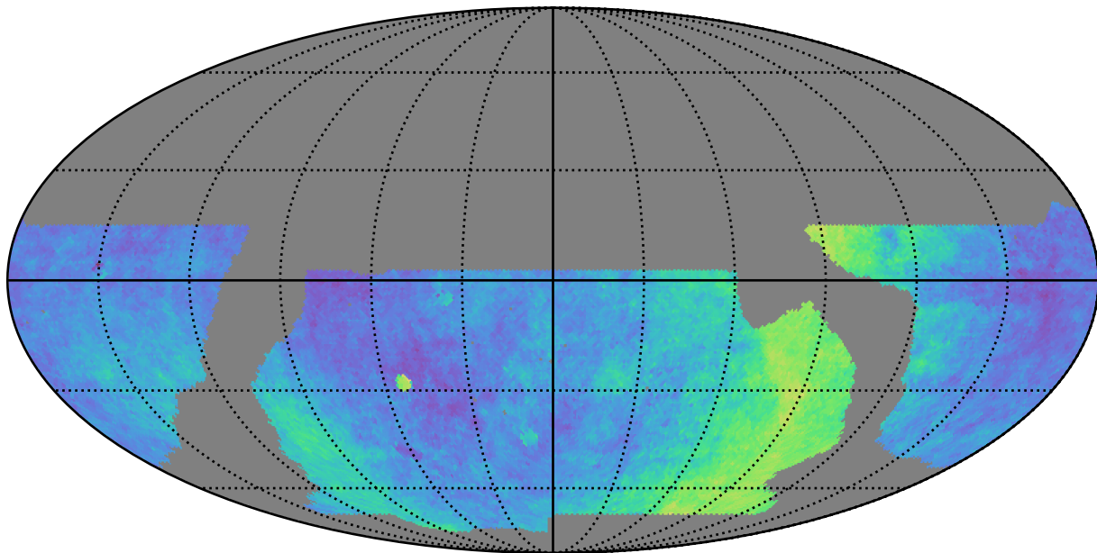
baseline_v2.1_10yrs WFD: Parallax Coverage @ 22.4
