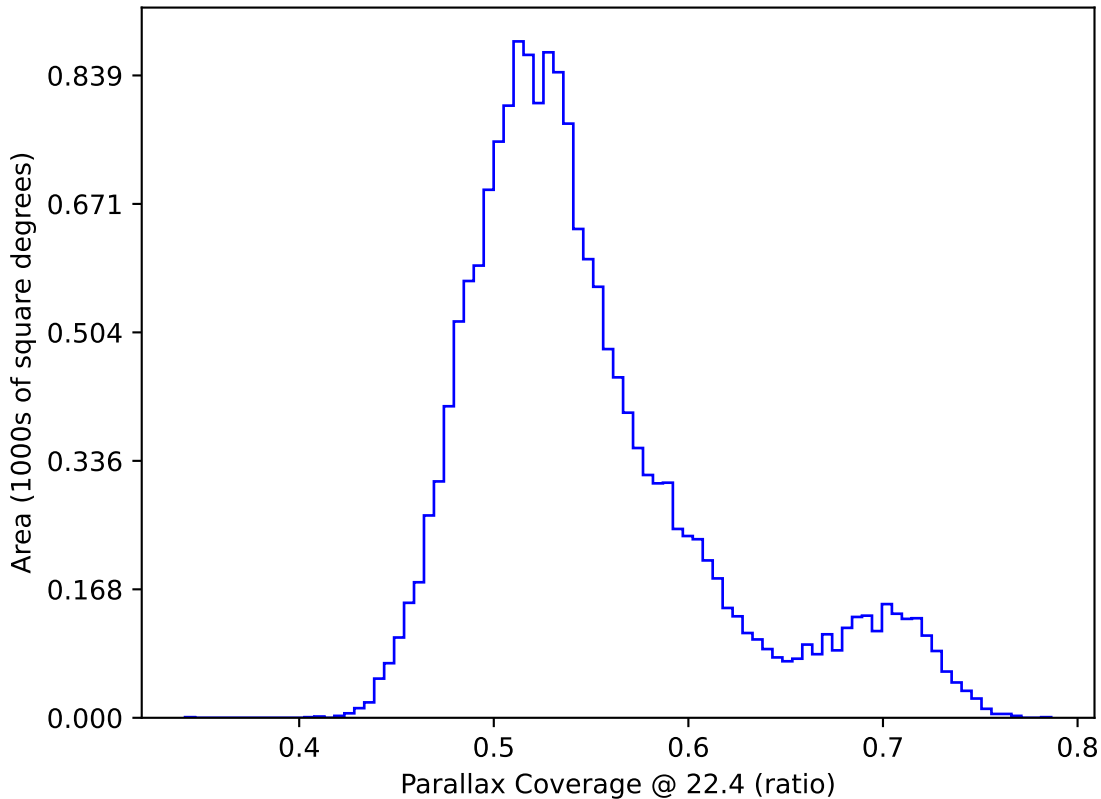
baseline_v2.1_10yrs WFD: Parallax Coverage @ 22.4
