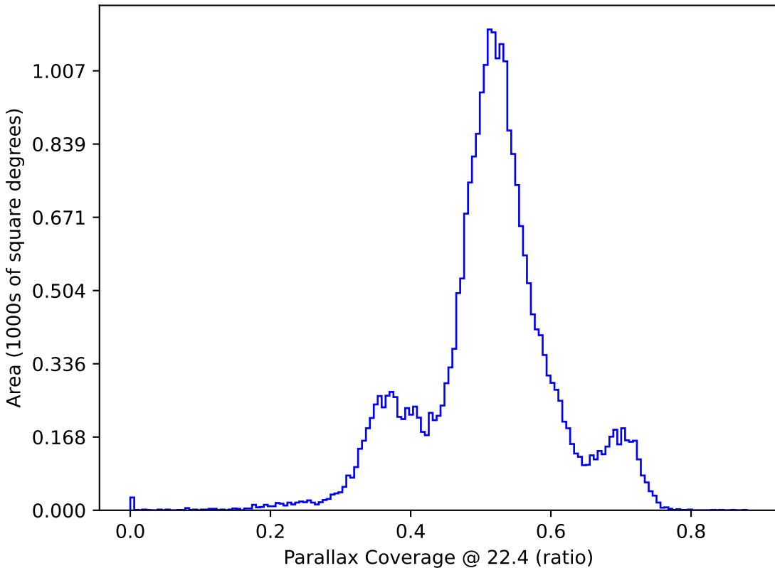
baseline_v2.1_10yrs All sky: Parallax Coverage @ 22.4
