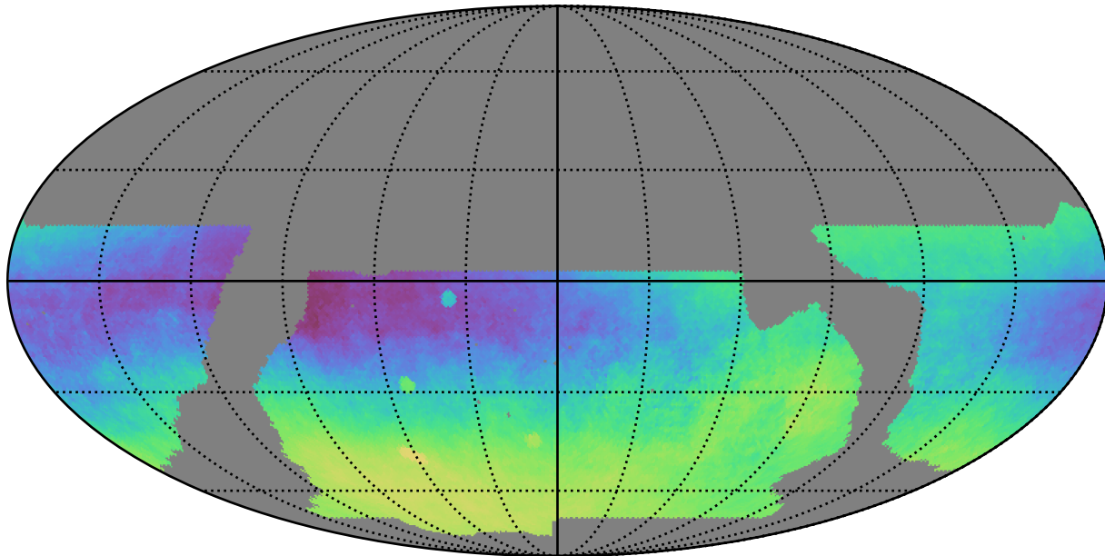
baseline_v2.1_10yrs WFD: Parallax-DCR degeneracy @ 24.0
