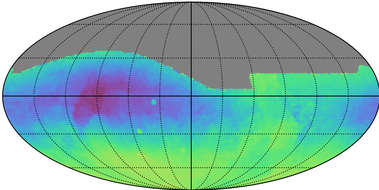
baseline_v2.1_10yrs All sky: Parallax-DCR degeneracy @ 24.0
