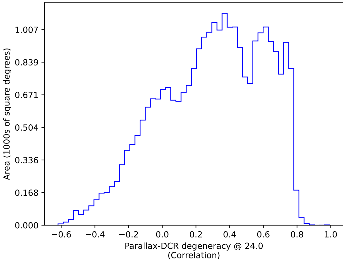
baseline_v2.1_10yrs All sky: Parallax-DCR degeneracy @ 24.0
