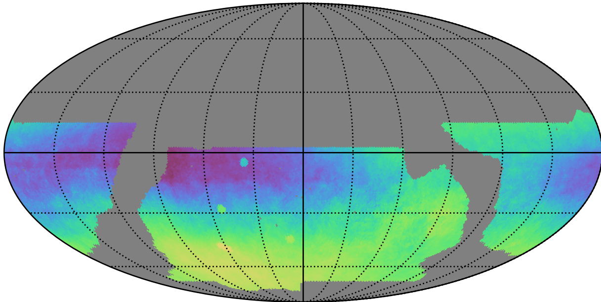
baseline_v2.1_10yrs WFD: Parallax-DCR degeneracy @ 22.4
