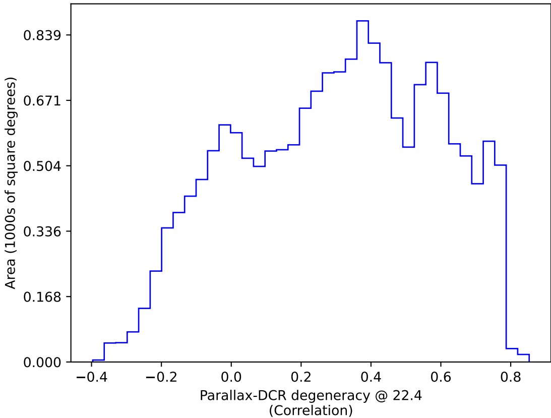
baseline_v2.1_10yrs WFD: Parallax-DCR degeneracy @ 22.4
