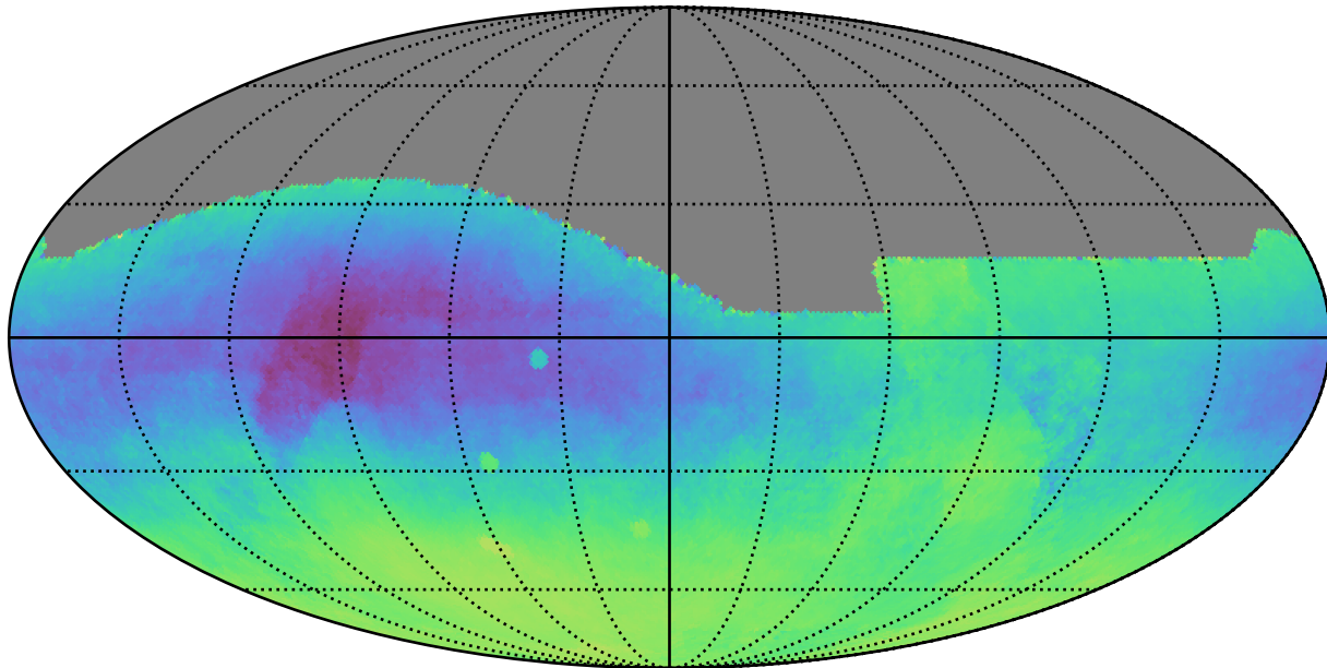
baseline_v2.1_10yrs All sky: Parallax-DCR degeneracy @ 22.4
