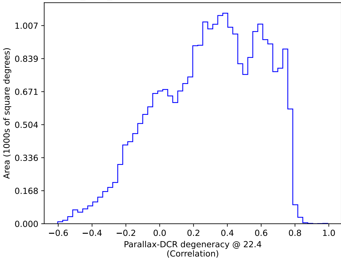
baseline_v2.1_10yrs All sky: Parallax-DCR degeneracy @ 22.4
