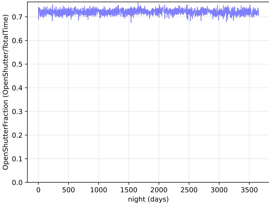
baseline_v2.1_10yrs Per night: OpenShutterFraction
