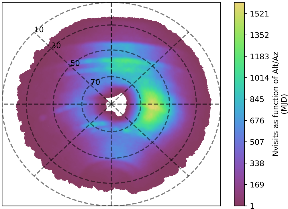
baseline_v2.1_10yrs z band: Nvisits as function of Alt/Az
