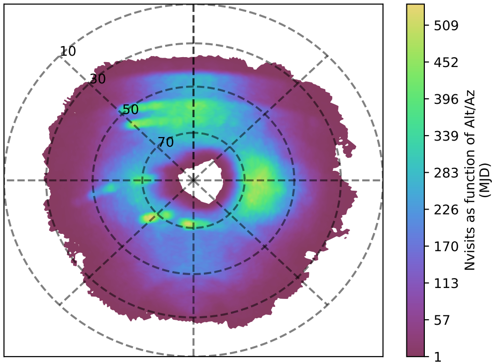
baseline_v2.1_10yrs u band: Nvisits as function of Alt/Az
