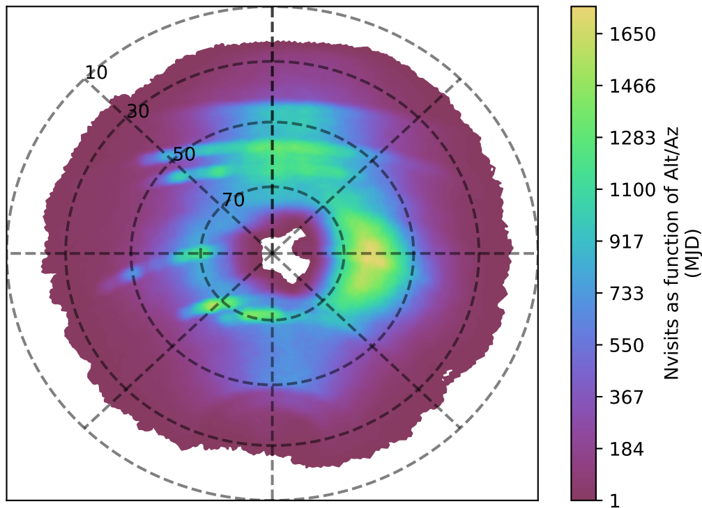
baseline_v2.1_10yrs r band: Nvisits as function of Alt/Az
