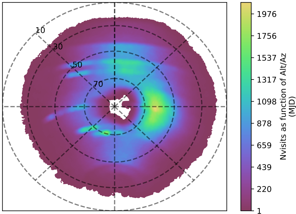
baseline_v2.1_10yrs i band: Nvisits as function of Alt/Az
