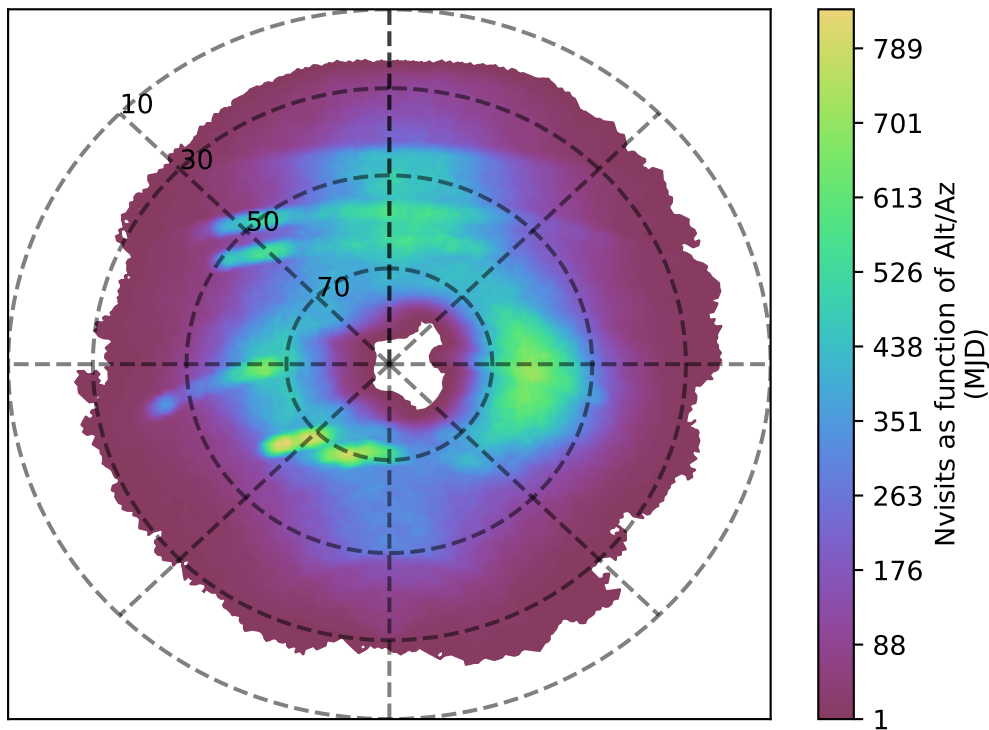
baseline_v2.1_10yrs g band: Nvisits as function of Alt/Az
