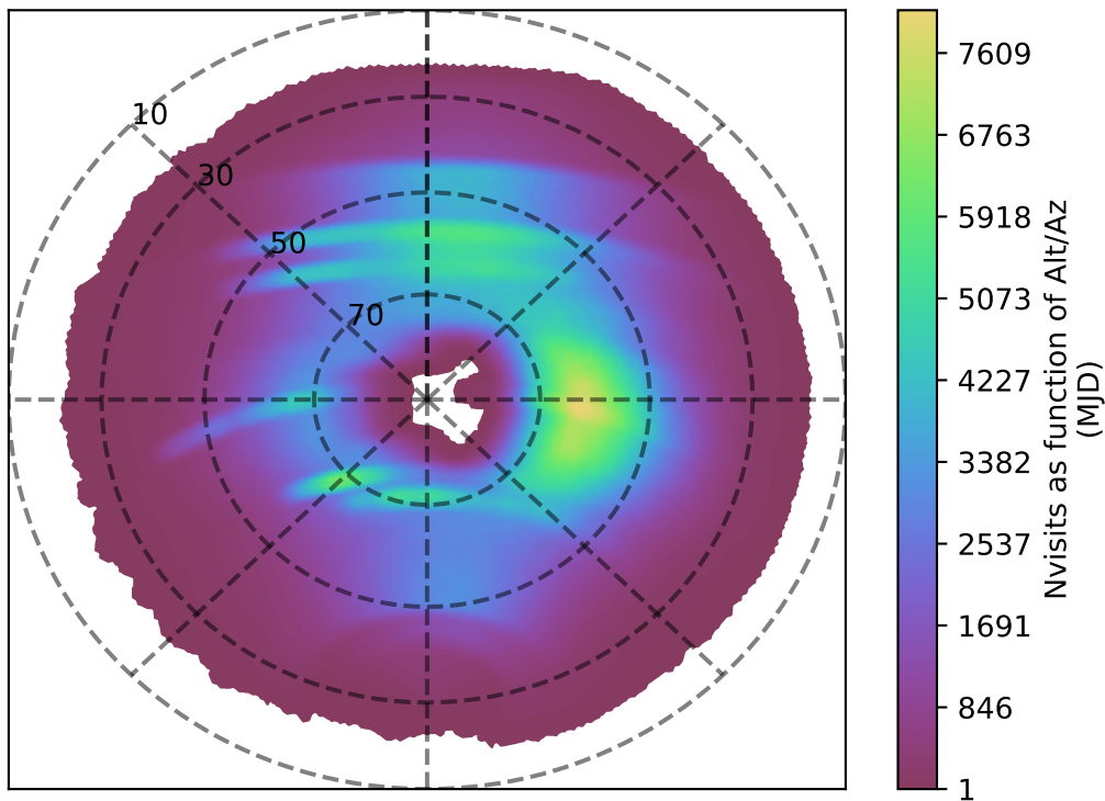
baseline_v2.1_10yrs all bands: Nvisits as function of Alt/Az
