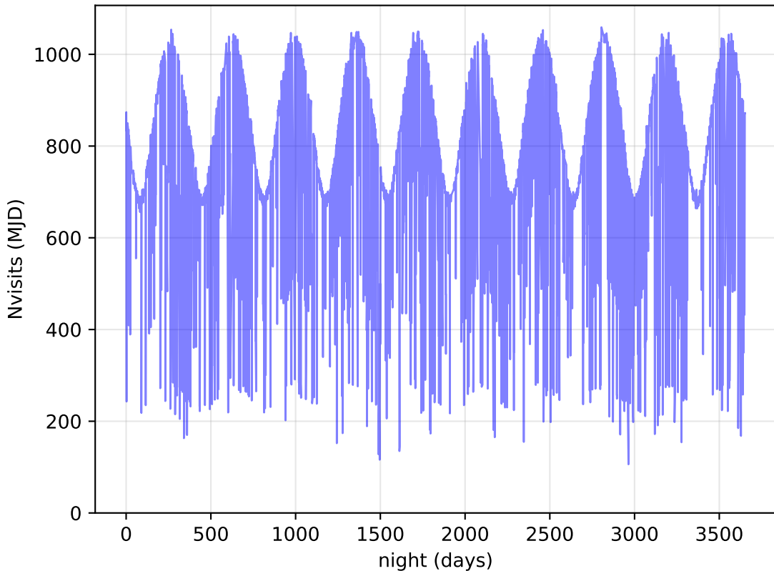
baseline_v2.1_10yrs All visits: Nvisits
