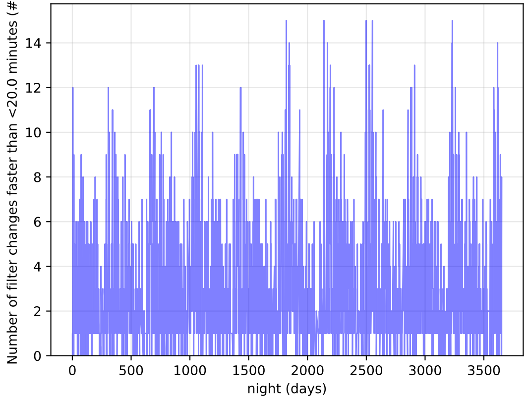
baseline_v2.1_10yrs Per Night: Number of filter changes faster than <20.0 minutes
