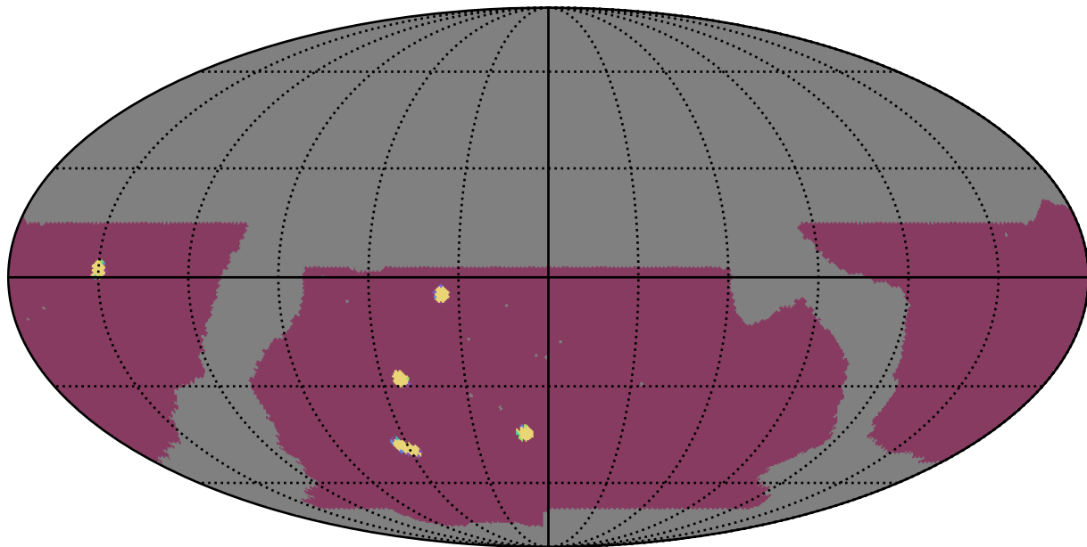
baseline_v2.1_10yrs WFD: NumberOfQuickRevisits
