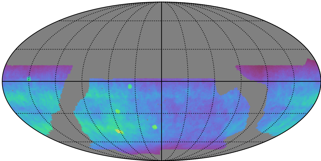
baseline_v2.1_10yrs WFD z band: Normalized Teff
