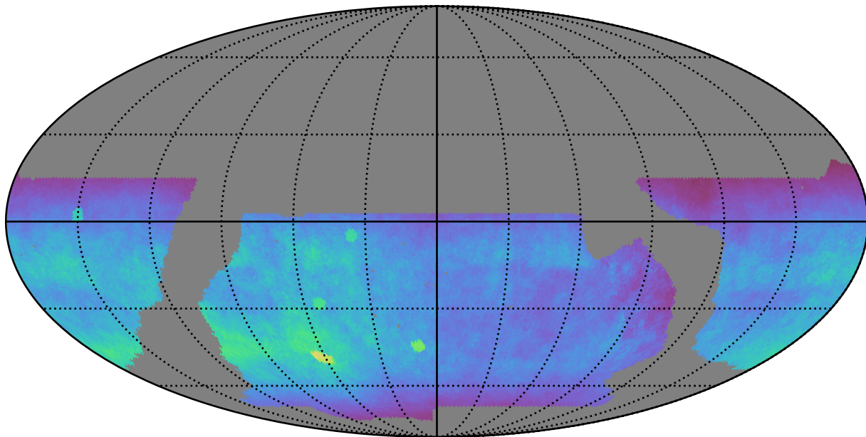
baseline_v2.1_10yrs WFD y band: Normalized Teff
