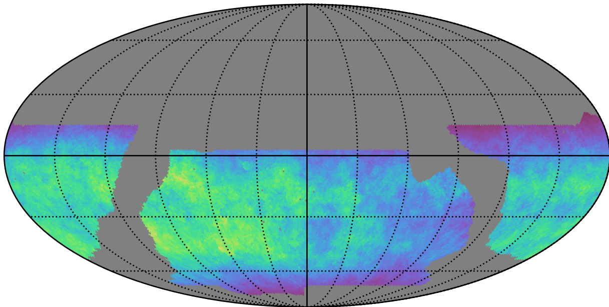
baseline_v2.1_10yrs WFD u band: Normalized Teff
