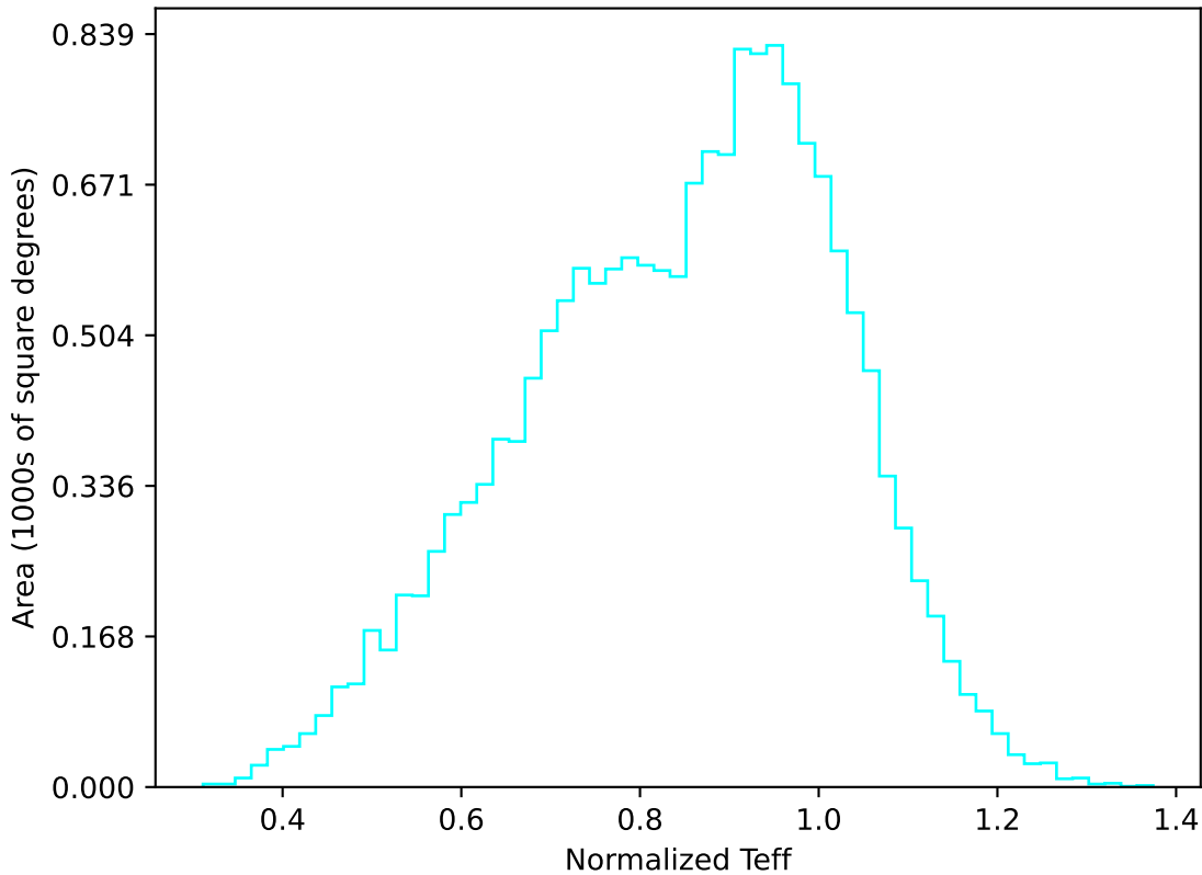
baseline_v2.1_10yrs WFD u band: Normalized Teff
