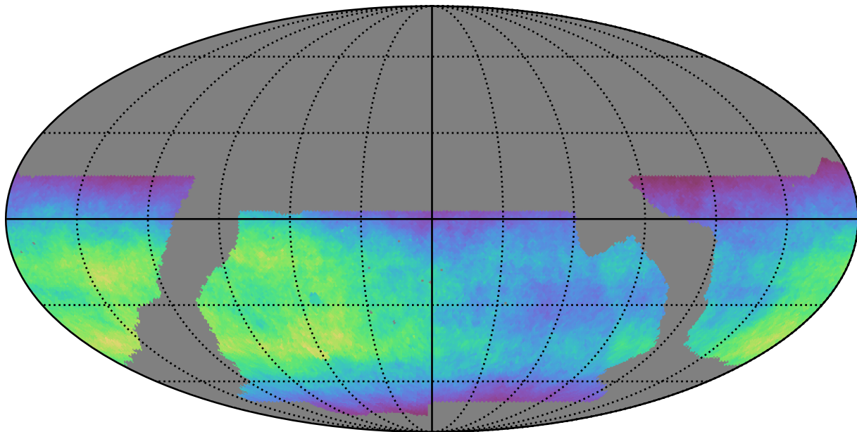
baseline_v2.1_10yrs WFD r band: Normalized Teff
