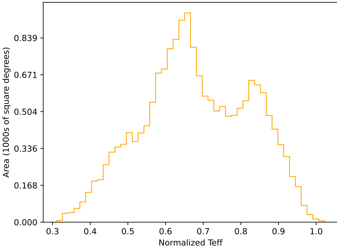
baseline_v2.1_10yrs WFD r band: Normalized Teff
